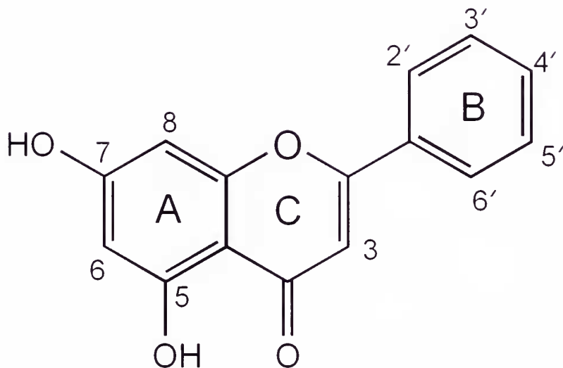
Figure 1: Flavones: 5,7,4'-OH=Apigenin; 5,7,3',4'-OH=Luteolin; 5,7,3',4',5'-OH=Tricetin. Flavonols: 3,5,7,4'-OH=Kaempferol; 3,5,7,3',4'-OH=Quercetin.
